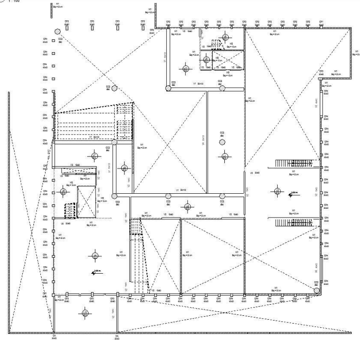
1 Floor Plan - S/PB 1:100
